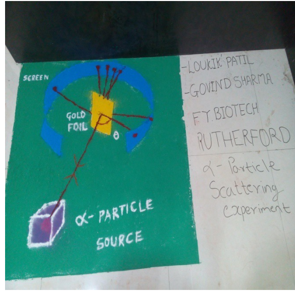
\alpha – particle scattering ( physics rangoli )
